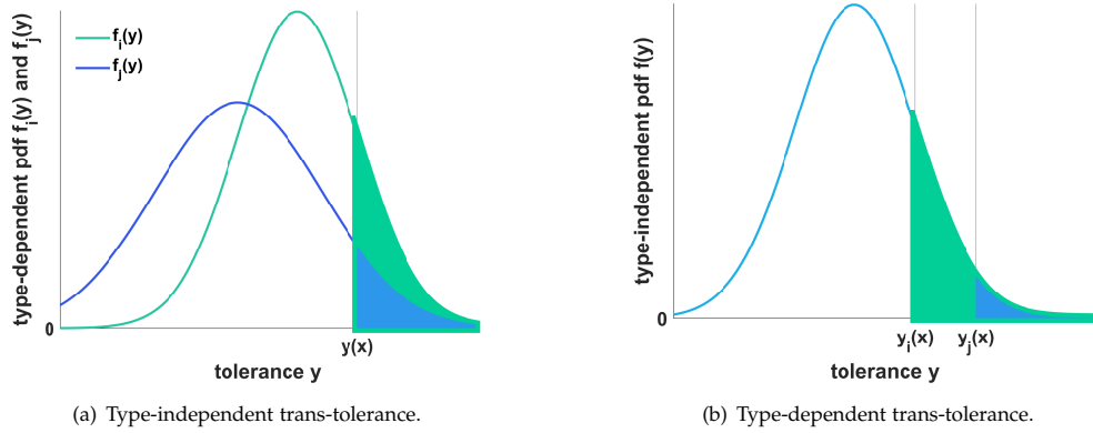
Figure 5. Shaded areas mark a measure of Chloe's. In either case, type i has more Chloe's than type j .
